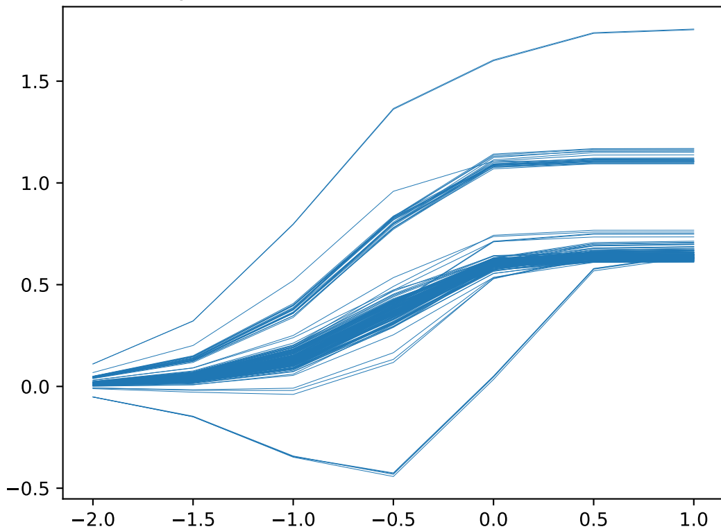
Dynamic Ricci Curvature for Geodesic 0.8
